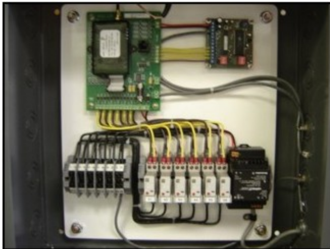
RCD- 6 EAS System With 1 Receiver, LED Sign and Audio Output.
